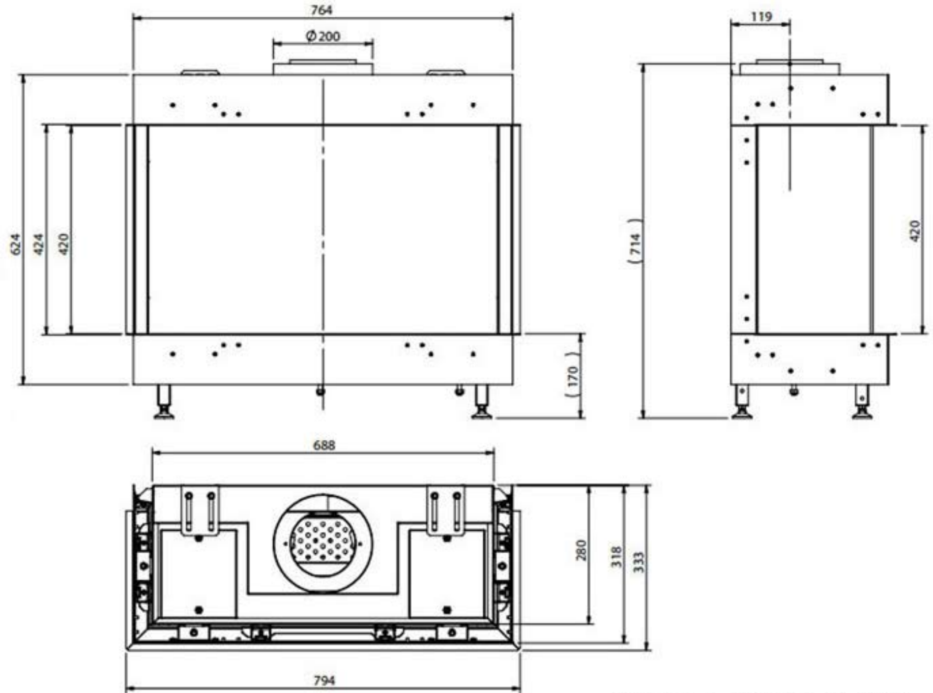
Three Sided 70
